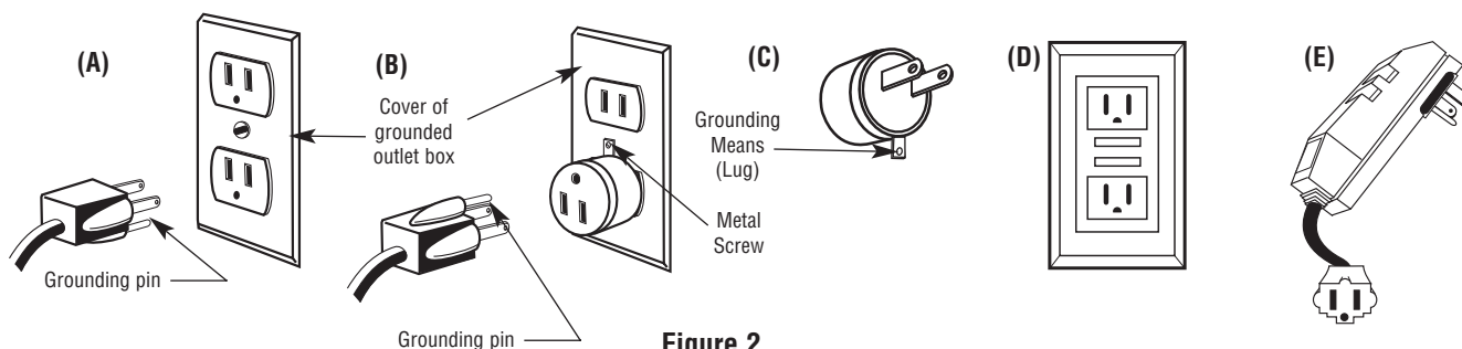
Figure 2 Grounding Methods
